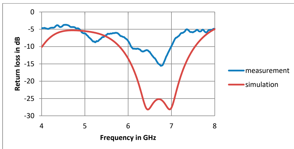
Figure 14. The simulated and measured return losses of the slot antenna (thickness = 1.27 mm).
