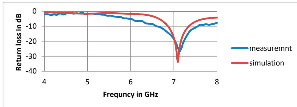
Figure 9. The simulated and measured return loss of antenna A with thickness of 0.508 mm.
