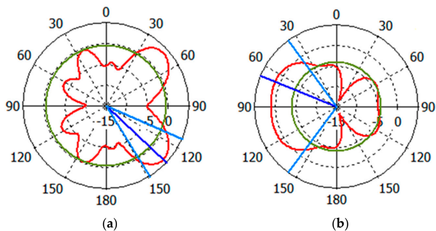
Figure 16. The radiation pattern of the bow-tie slot antenna (a), E-plane and H-plane (b).
