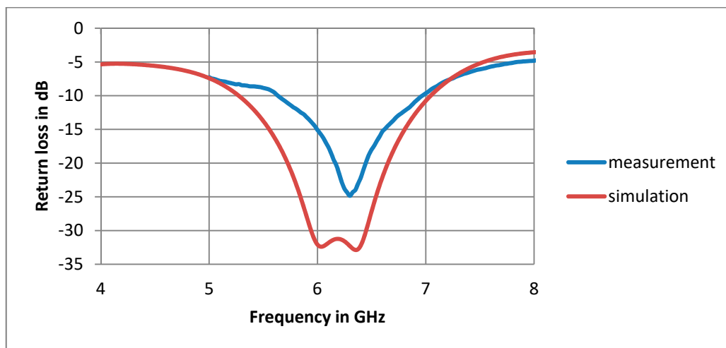
Figure 15. The simulated and measured return losses of the slot antenna (thickness = 0.508 mm).
