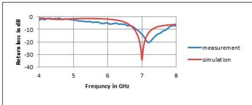
Figure 7. The comparison of simulated and measured return loss of antenna B.
