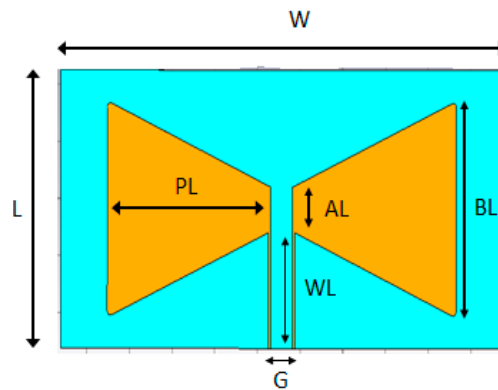
Figure 1. The design geometry of antenna A and B with same RT/Duroid 5880 materials substrate and different substrate thickness.
