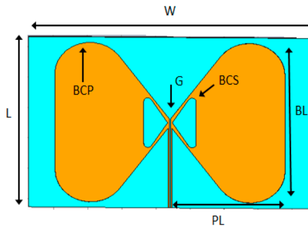
Figure 3. The geometry of the proposed broadband antenna.
