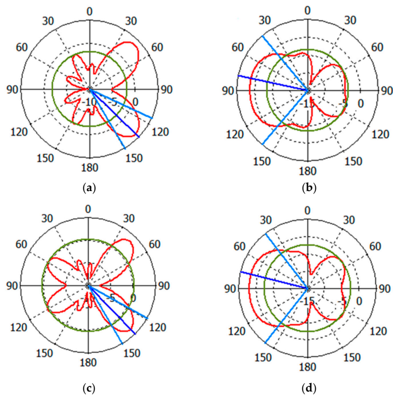
Figure 11. The radiation pattern of the proposed antennas (a), E plane of antenna A (b), H plane of antenna A (c), E plane of antenna B (d) and H plane of antenna B.
