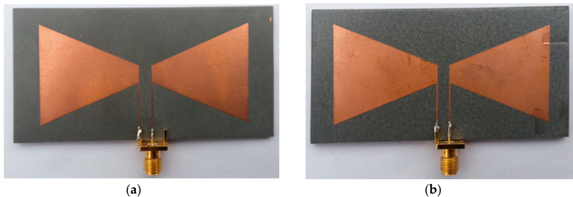
Figure 4. Fabricated bow-tie (a) antenna A with a thickness of 1.57 mm and 0.508 mm, (b) antenna B with a thickness of 3.175 mm and 1.27 mm.
