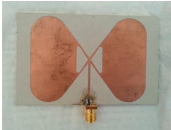
Figure 5. Image of the fabricated wideband bow-tie antenna.
