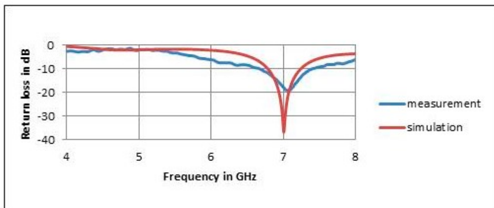
Figure 6. The comparison of simulated and measured return loss of antenna A.
