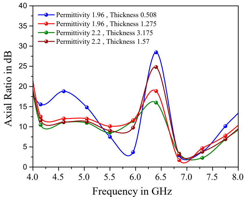
Figure 13. Simulated axial ratios of the antennas over the frequency range of interest.
