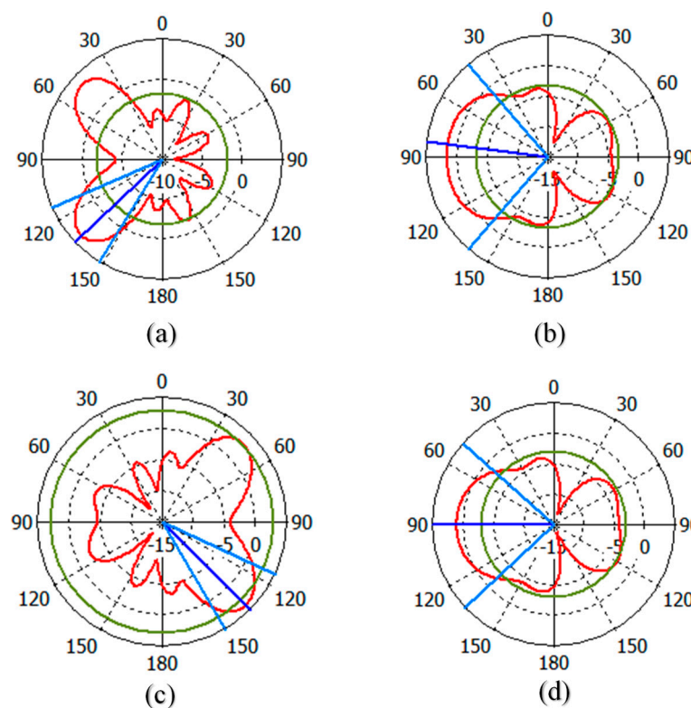
Figure 8. The radiation pattern of the proposed antennas (a): E plane of antenna A (b), H plane of antenna A (c), E plane of antenna B (d), and H plane of antenna B (b).
