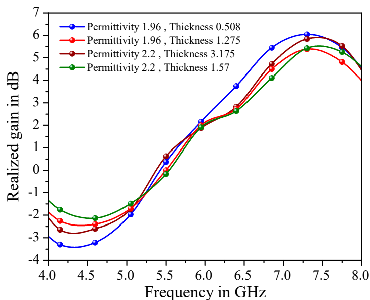
Figure 12. Realized gain of the proposed antennas versus the frequency in the range of interest.
