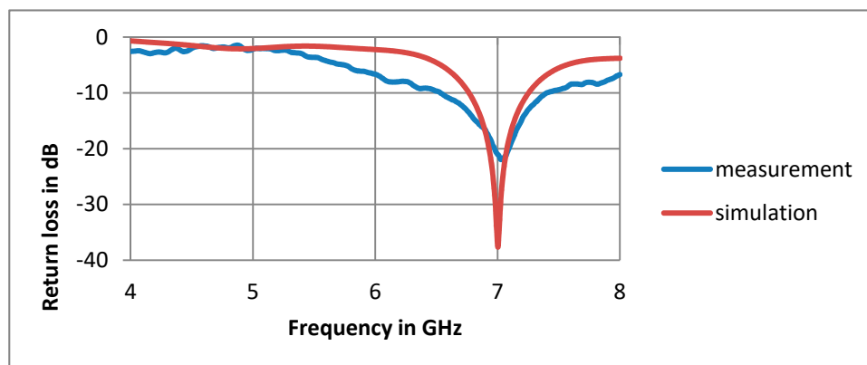
Figure 10. The simulated and measured return loss of antenna B with thickness of 1.27 mm.
