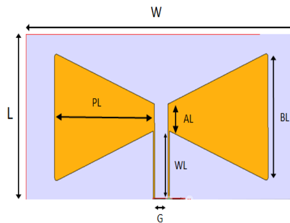
Figure 2. Design of the geometry of antenna A and B with same substrate RT/Duroid 5880LZ material and different thickness.
